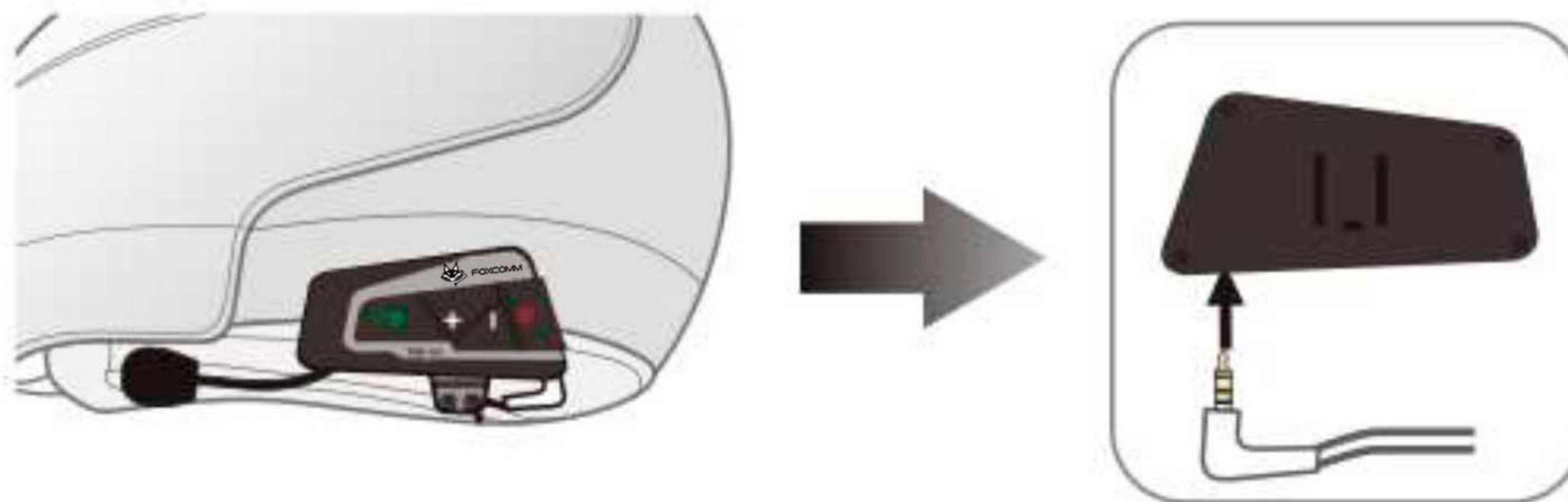
⑥ Insert the headphone plug into the corresponding headphone jack on the receiver to finish the installation.
